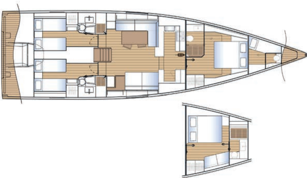
INTERIOR PLAN
