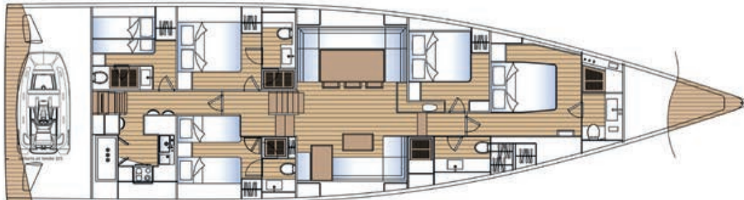
ALTERNATIVE INTERIOR PLAN
